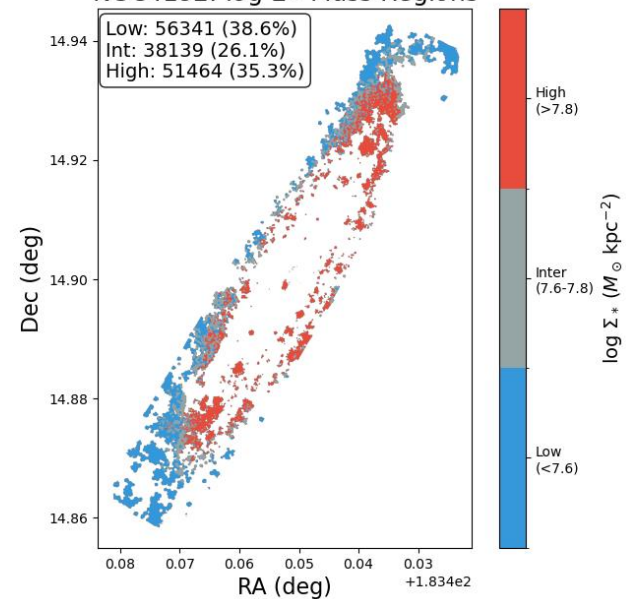
NGC4192: \log \Sigma_{*} Mass Regions
