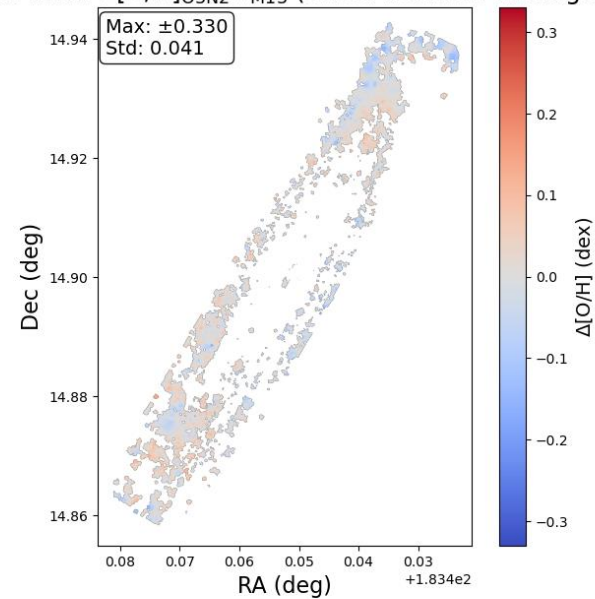
NGC4192: \Delta[\text{O}/\text{H}]_{\text{O3N2}-\text{M13}} (offset from bin average)
